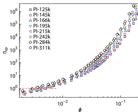
Fig. 5 Plot of specific viscosity \eta_{sp} against \phi for PI samples with different molecular weights at 20 °C.
