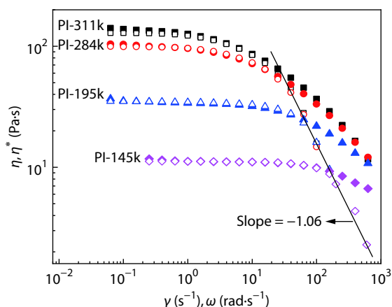
Fig. 4 Cox-Merz plot of PI in DMF with different molecular weights at \phi = 0.120 and 20 °C. \eta^* and \eta are represented by filled and hollow symbols, respectively. Solid line represents the power-law relationship.
