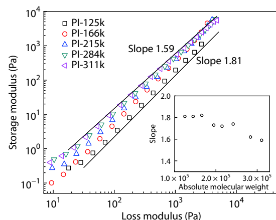
Fig. 3 The log-log plot of storage modulus G' versus loss modulus G'' of PI samples with different molecular weights at \phi = 0.120 and 20 °C. The inset shows the variation of slope with molecular weight.
